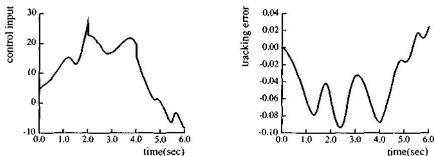
Figure 7.12a : Control input and resulting tracking performance
