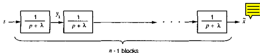
Figure 7.1.a : Computing bounds on \tilde{\mathbf{x}}
